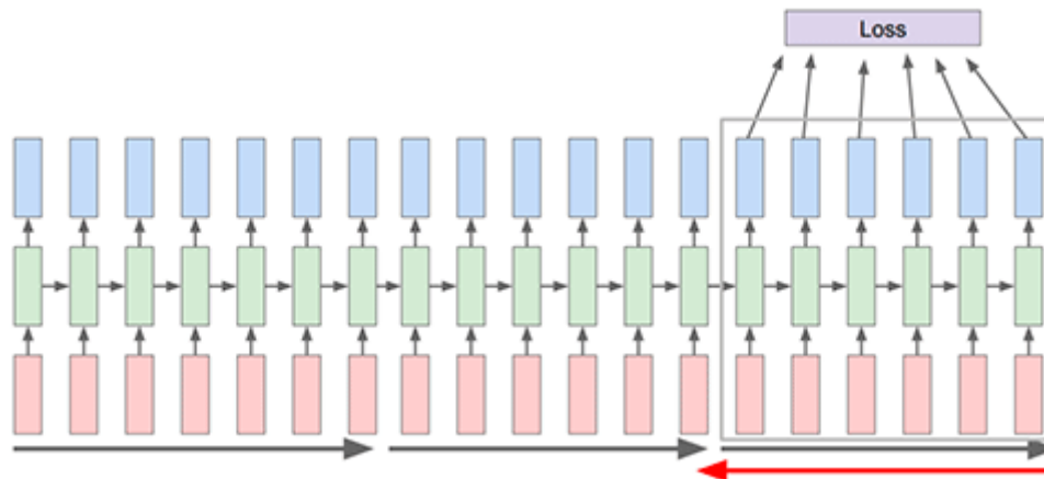
Figura 10. Truncated Backpropagation Through Time (TBPTT) .
